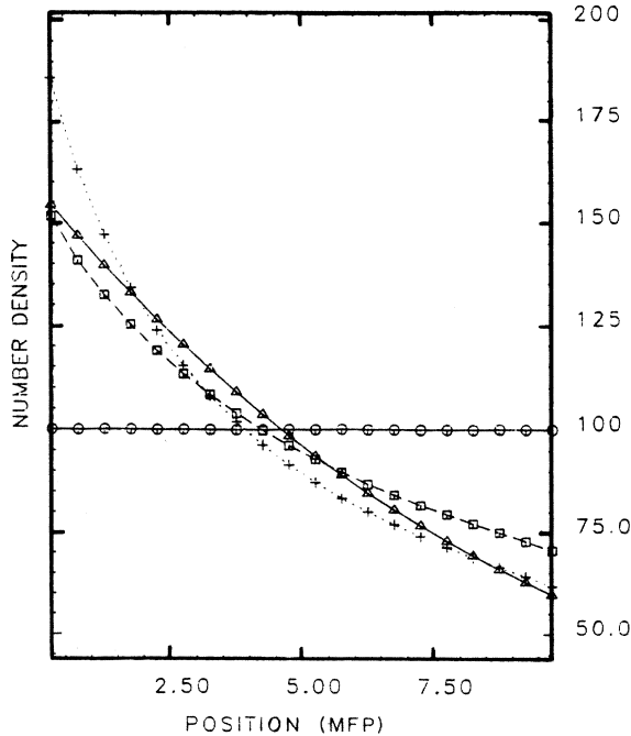
FIG. 1. Plot of number density as a function of cell position. Position is measured in units of mean free path. The solid line with circles is for the equilibrium system ( T_1=T_2=1 ) without gravity; the solid line with triangles is for the equilibrium system with gravity. The dashed line with squares is for a temperature gradient of T_1=1, T_2=3 . The dotted line with crosses is for a gradient of T_1=1, T_2=5 .
