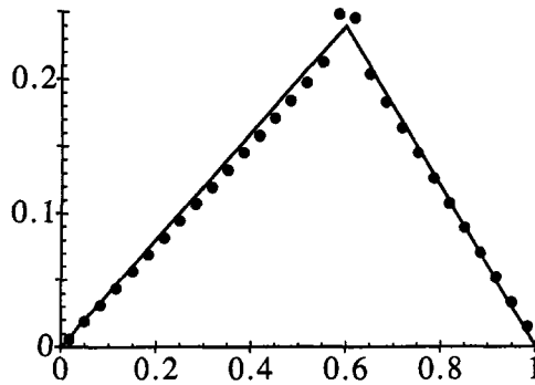
Fig. 1. Correlation of reduced temperature fluctuations \overline{\langle \delta T(z) \delta T(z') \rangle} versus z'/L as given by Eq. (8) (filled circles) and by Eq. (7) (solid line) for z/L = 0.6 . The parameters are set so that (T_L - T_0)^2 k_B / (\rho C_p L_x L_y L_z) = 1 .
